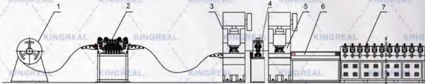
1. Decoiler 2. Precision Straightener 3. Press 1 4. Servo feeder 5. Press 2 6. Conveyor 7 Roll Forming Station
